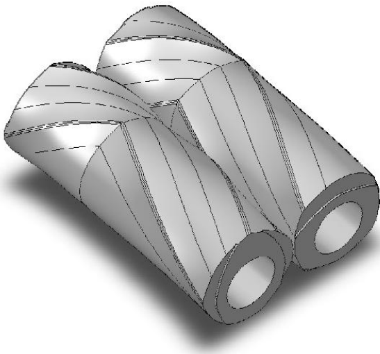
Figure 7. Mixing Elements using Fractional Lobed profile offered highest level of Shear uniformity and Intensity
