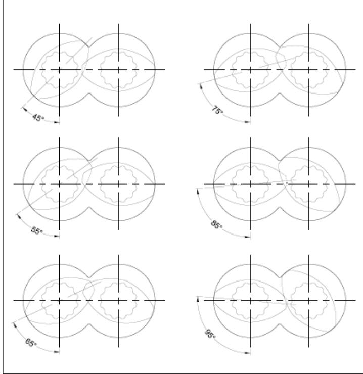
Figure 4. Development of Meta-radial shear in Bi-lobed Kneading blocks
