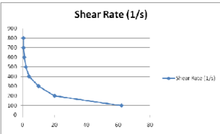
Figure 3. Radial shear rate for Fractional Four lobe profile
