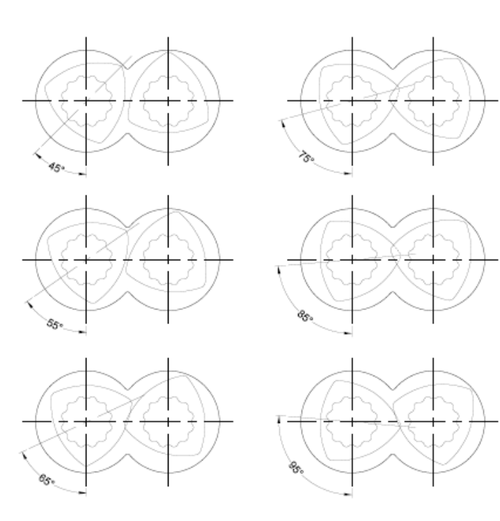
Figure 5. Development of Meta-radial shear in Eccentric tri-lobed Kneading blocks
