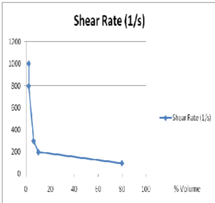
Figure 1. Radial shear rate for bi-lobed profile at 400 RPM
