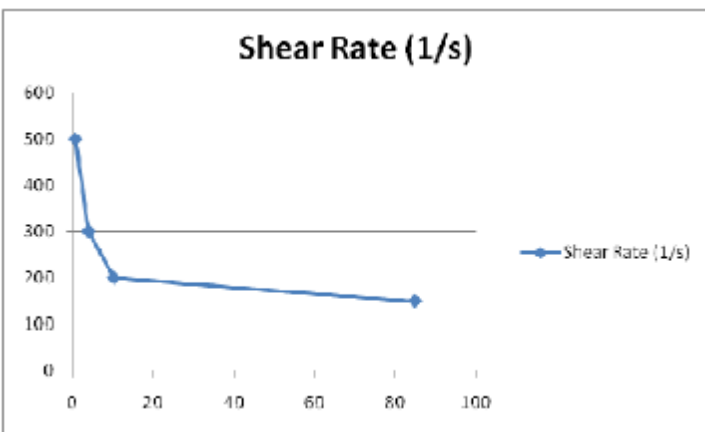
Figure 2. Radial shear rate for eccentric tri-lobed profile
