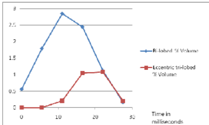
Figure 6. Volume Fraction subjected to intense shear rate of 1400 1/s @ 400 RPM
