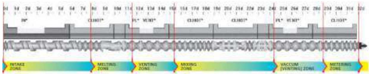
Figure 3: Process Zone in a Co-rotating twin-screw extruder
