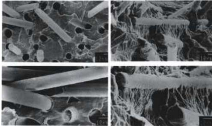
Figure 1: SEM Pictures of Glass Fiber Wetting & Coupling
